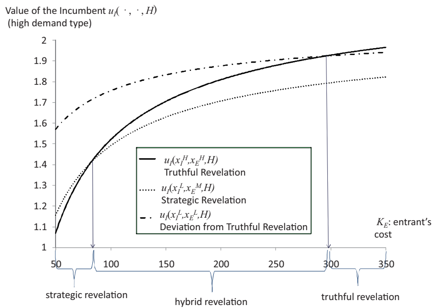
Figure 5: Values of the high-demand u_I(\cdot, \cdot, H) , high-cost K_E incumbent
